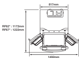
Drawer-Type
