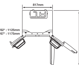
Swing-Type
